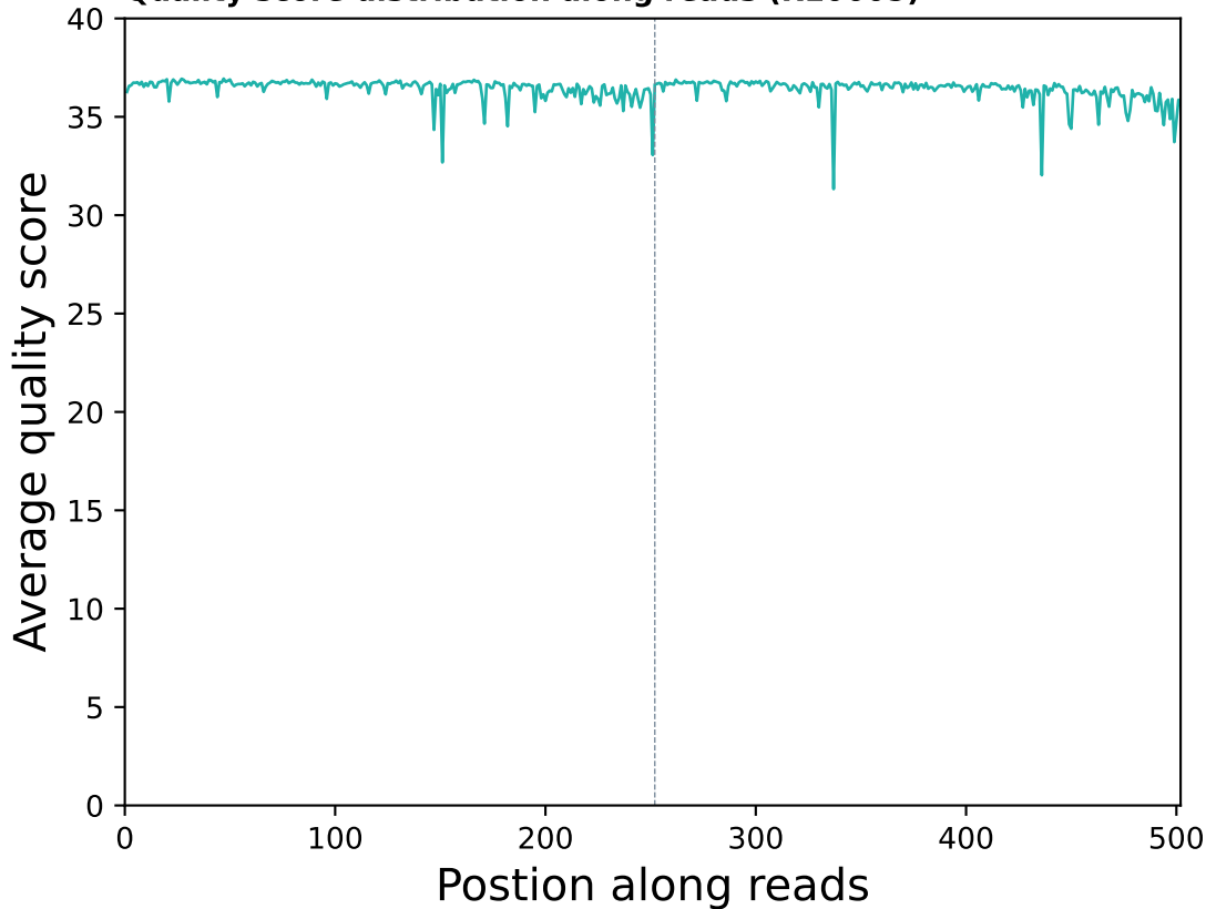
Quality score distribution along reads (R10605)
